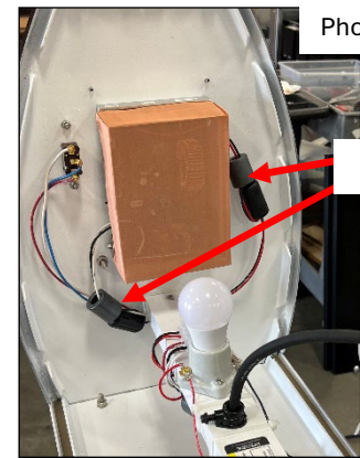
Ferrites
