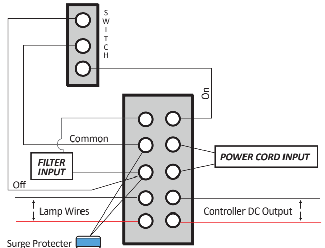
LED Sign - SWITCH
