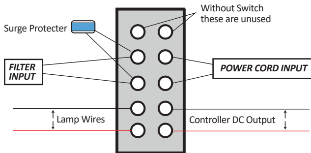
LED Sign - NO SWITCH
