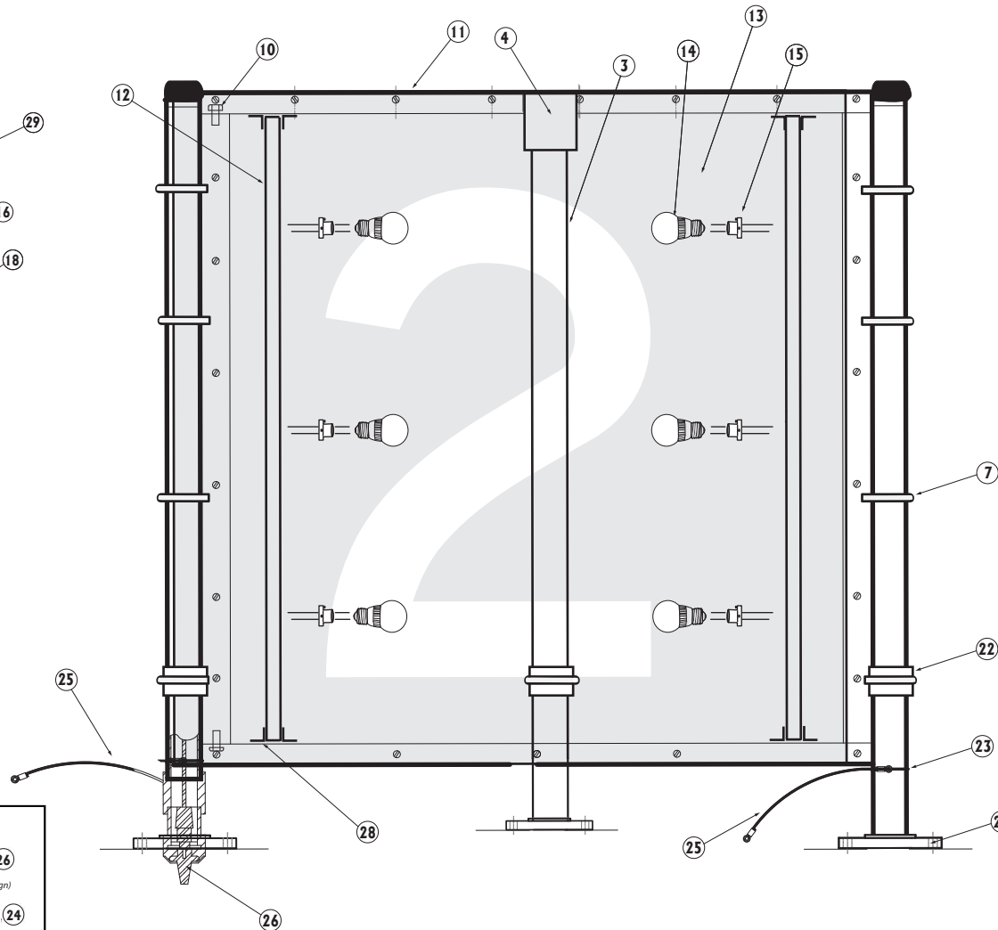
Inside Electrical View
