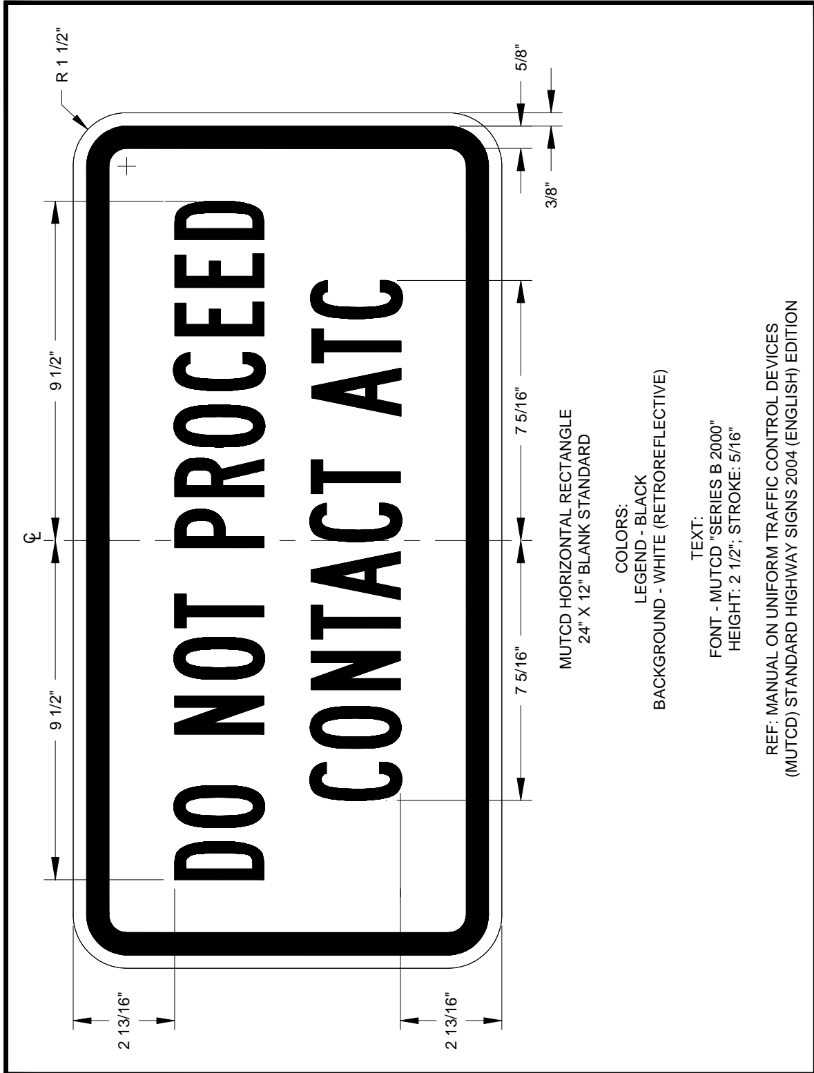
Figure 14c. DO NOT PROCEED Sign Detail.
