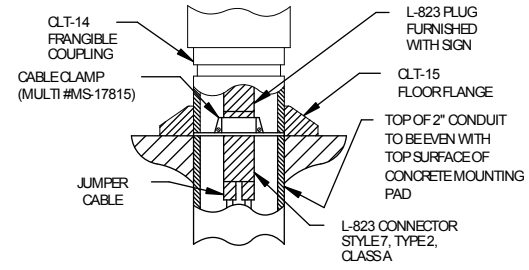
ELECTRICAL CONNECTION DETAIL
